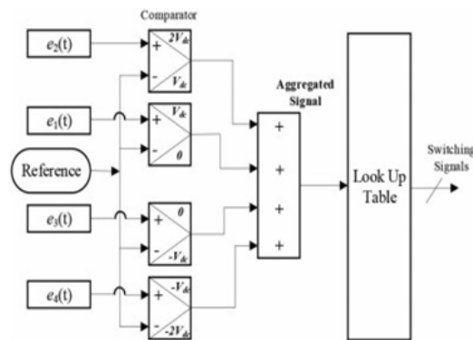
Fig. . Switching signal generation schematic diagram pattern of the switches.
